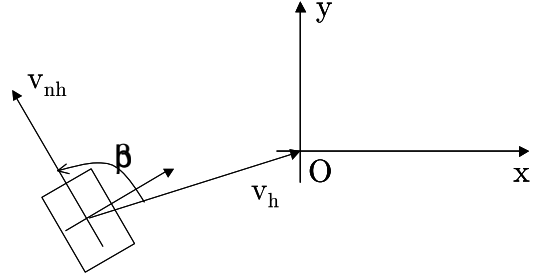
Fig. 5. Holonomic and nonholonomic velocities
